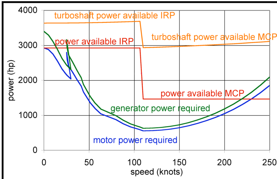
Figure 3. Tilting power requirements vs. speed. 4
