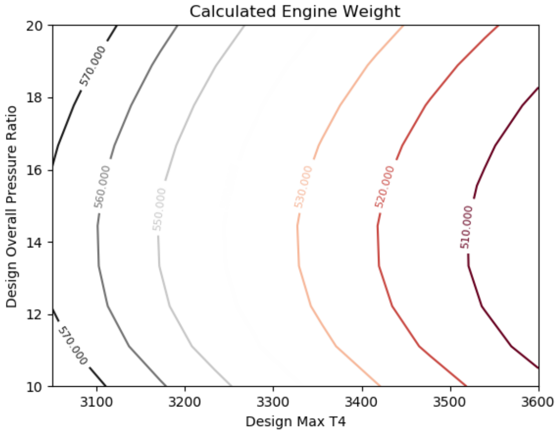
Figure 9. Calculated engine dry weight, lbm.
